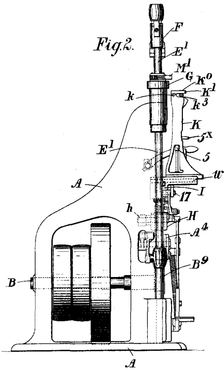
17660 United Shoe Machinery Company. Heel-attacher. (Bates.)
