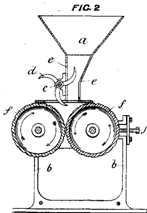
17797 Hay and Daniel. Treating Offal.
