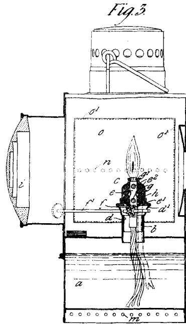
18861 The Lamp Manufacturing Company (Limited). Signal-lamp. (Welch.)
