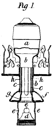
18853 Alexander. Gas-burner.
