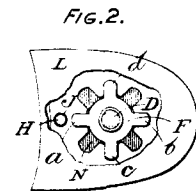
18903 McCubbin. Boot-heel.
